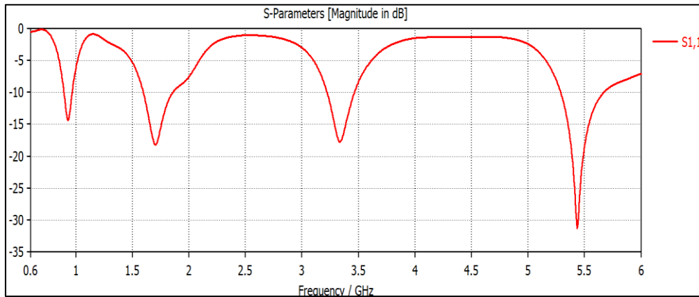
Fig. 2: Return loss of proposed antenna
