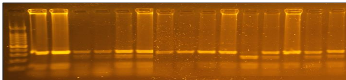
Figure 2. DNA fragment digestion with BsmA1 restriction enzyme
