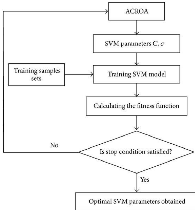
Fig. 4: Flow chart of SVM algorithm
