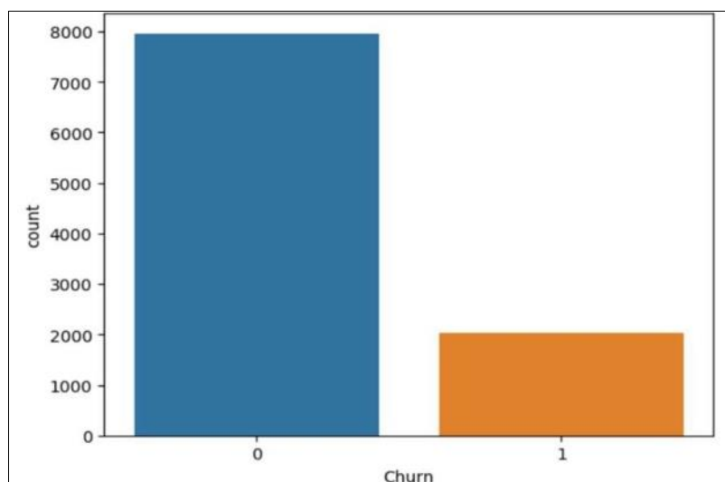
Fig. 1: Imbalanced data
