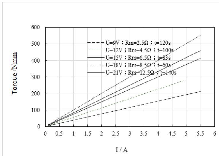
Figure 6: Relations of simulation torque and current under different motor resistance R_m , t and U
