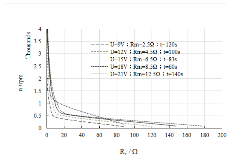
Figure 5: Relations of simulation rotation and resistance R_v under different motor resistance R_m , t and U
