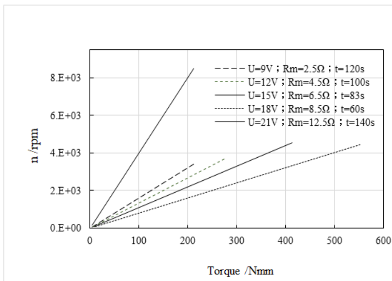
Figure 8: Relations of simulation torque and rotation under different motor resistance R_m , t and U
