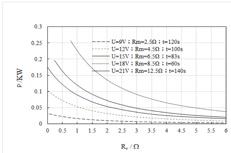
Figure 3: Relations of simulation power and resistance R_v under different motor resistance R_m , t and U
