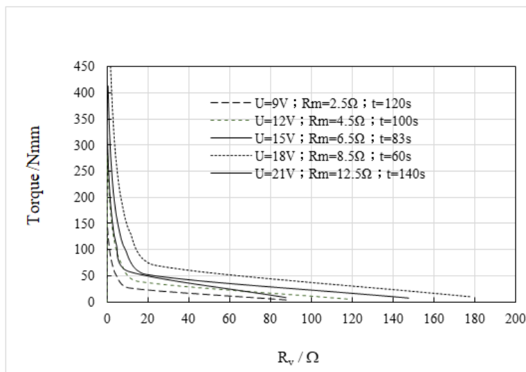
Figure 7: Relations of simulation torque and resistance R_v under different motor resistance R_m , t and U
