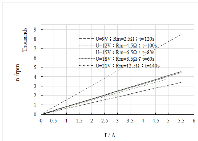
Figure 4: Relations of simulation rotation and current under different motor resistance R_m , t and U
