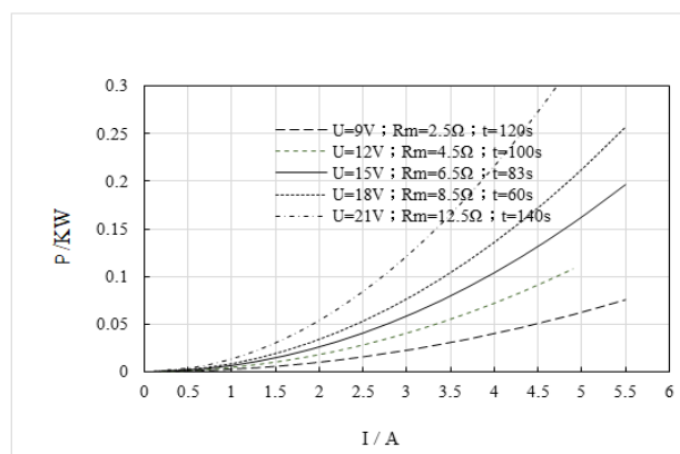
Figure 2: Relations of simulation power and current under different motor resistance R_m , t and U
