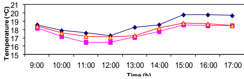
◆ Ambient Temperature ■ Bottom Temperature ▲ Top Temperature ( T_{\text{indoor}} ) ( T_{\text{bottom}} at 50 cm) ( T_{\text{top}} at 150 cm). Appendix 2.9. Temperature variation in June.
