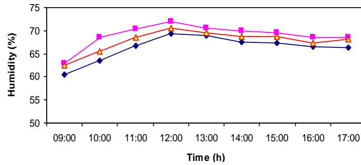
◆ Ambient Humidity ■ Bottom Humidity ▲ Top Humidity ( H_{\text{indoor}} ) ( H_{\text{bottom}} at 50 cm) ( H_{\text{top}} at 150 cm). Appendix 2.10. Average daily variation of humidity in June.
