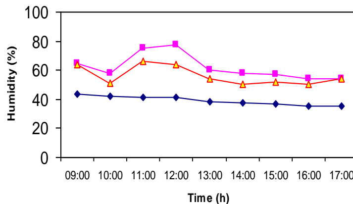
◆ Ambient Humidity ■ Bottom Humidity ▲ Top Humidity ( H_{\text{indoor}} ) ( H_{\text{bottom}} at 50 cm) ( H_{\text{top}} at 150 cm). Appendix 2.12. Average daily variation of humidity in July.
