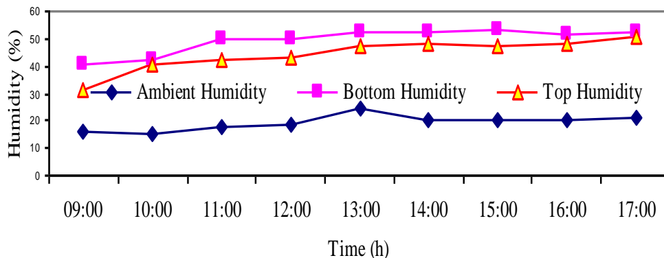
( H_{indoor} ) ( H_{bottom} at 50 cm) ( H_{top} at 150 cm). Appendix 2.18. Average daily variation of humidity in October.
