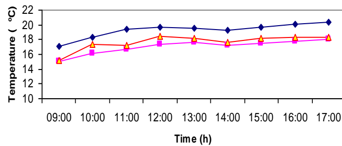
◆ Ambient Temperature ■ Bottom Temperature ▲ Top Temperature ( T_{\text{indoor}} ) ( T_{\text{bottom}} at 50 cm) ( T_{\text{top}} at 150 cm). Appendix 2.11. Temperature variation in July.
