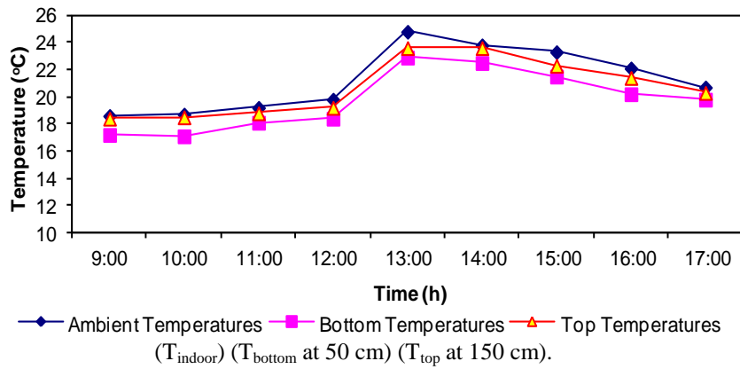
Appendix 2.3. Temperature variation in February.
