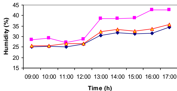
◆ Ambient humidity ■ Bottom humidity ▲ Top Humidity ( H_{\text{indoor}} ) ( H_{\text{bottom}} at 50 cm) ( H_{\text{top}} at 150 cm).
