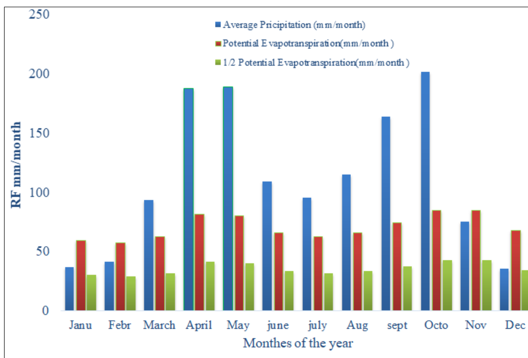
Figure 1: Fain fall distribution throughout the year at the study area starting from (2013-2023).
